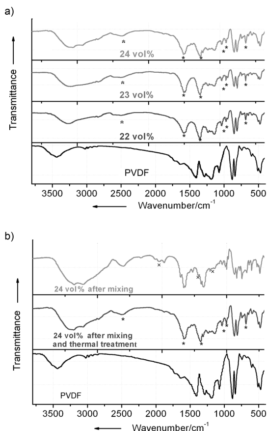
Figure 4. a) FTIR spectra of the samples containing 22–24 vol% \text{K}_2\text{CO}_3 before thermal treatment (pure PVDF is shown for comparison). b) FTIR spectra of the samples containing 24 vol% \text{K}_2\text{CO}_3 (pure PVDF is added for comparison). An asterisk and a cross locate the peaks of \text{KHCO}_3 and \text{KHF}_2 , respectively.
