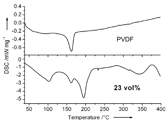
Figure 6. DSC curves of pure PVDF and composite sample containing 23 vol% \text{K}_2\text{CO}_3 .
