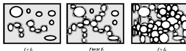
Figure 2. The formation process of the conductive network (dark gray) and its successive annihilation at the interface between PVDF (pale gray) and K_2CO_3 (white) with increasing the concentration of K_2CO_3 .
