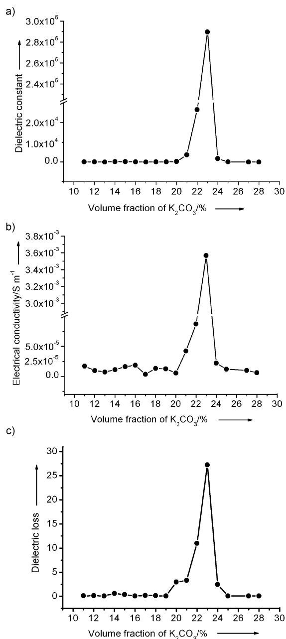
Figure 1. Variations of a) dielectric constant \epsilon_r , b) conductivity \sigma , and c) dielectric loss \tan\delta of PVDF- K_2CO_3 composites (at 10^3 Hz) as a function of volume fraction of K_2CO_3 .
